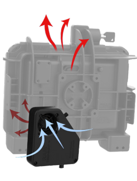
RAM-DOCK-HEATER1-EU RAM® Temp-Right™ Dock Heating Module for Zebra ET6x
