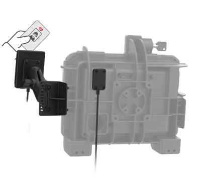
RAM-B-102-NFCU RAM® NFC Extender with Double Ball Mount
