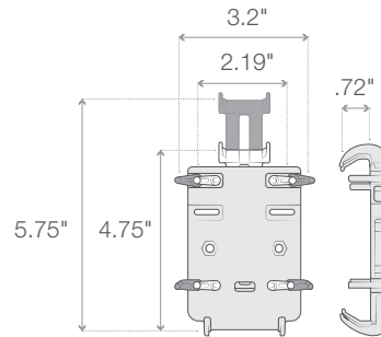
RAM-HOL-PD3-238AU Small Phone Holder with Ball
