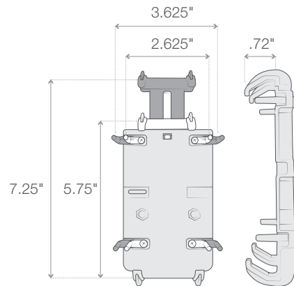
RAM-HOL-PD4-238AU Large Phone Holder with Ball
