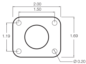
RAM-B-347U RAM-347U
