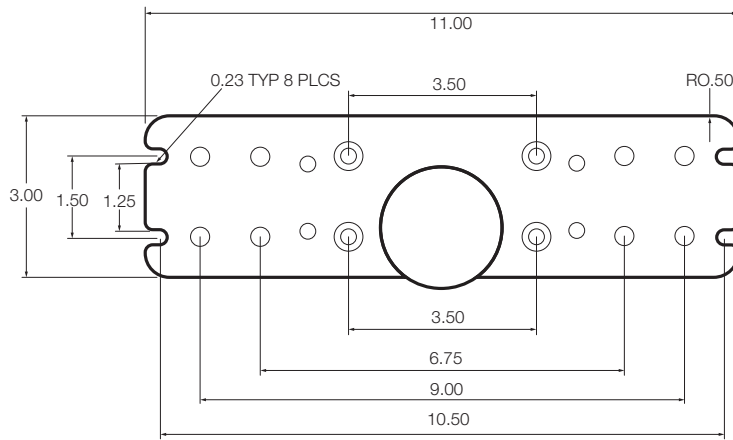
RAM-D-111BU
