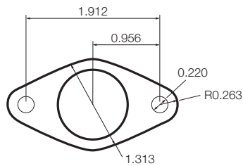
RAM-B-238U RAM-238U
