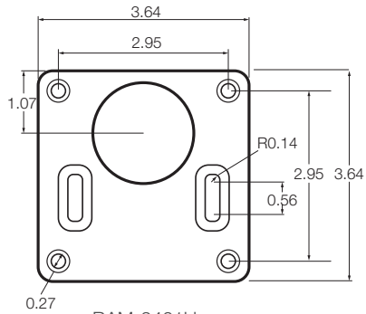
RAM-2461U RAM-D-2461U
